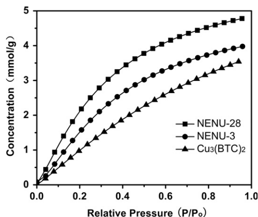
Fig. 4. Ethanol adsorption isotherms at 298 K for NENU-28, NENU-3, and \text{Cu}_3(\text{BTC})_2 .
