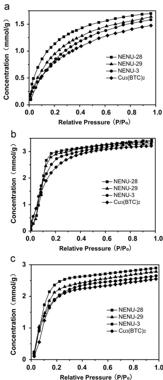
Fig. 9. Cyclohexane (a), benzene (b), and toluene (c) adsorption isotherms at 298 K for NENU-28, NENU-29, NENU-3, and \text{Cu}_3(\text{BTC})_2 .
