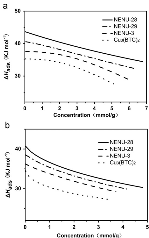
Fig. 7. Methanol (a) and ethanol (b) adsorption enthalpies for NENU-28, NENU-29, NENU-3, and \text{Cu}_3(\text{BTC})_2 .
