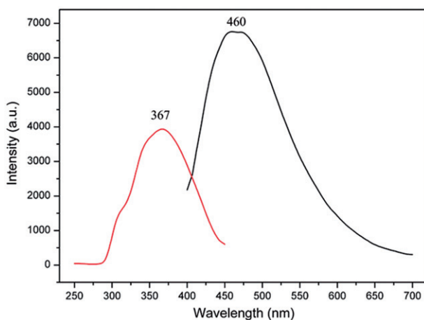
Figure 3. The excitation (left) and emission (right) spectra of 1 .
