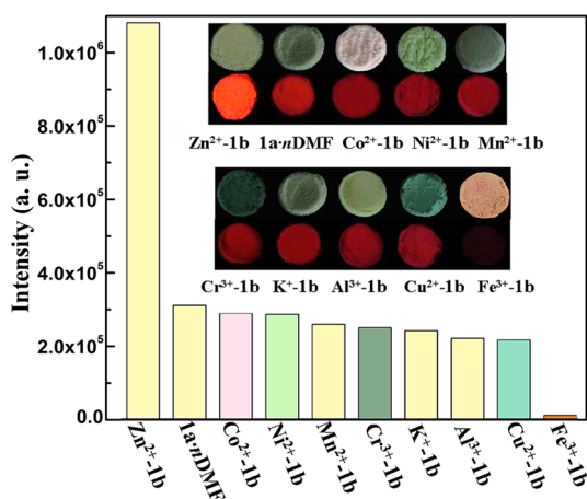
Figure 2. Comparison of the luminescence intensity of the ^5\text{D}_0 \rightarrow ^7\text{F}_2 transition of \text{M}^{z+}\text{-1b} versus 1a \cdot n\text{DMF} ( \lambda_{\text{ex}} = 344 nm). The inset shows the photographs of \text{M}^{z+}\text{-1b} under light and UV-light irradiation.
